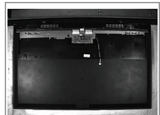
Large part positioning, orientation to robots, LCD panel
