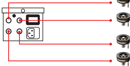
SE-CAB-AC-1: Non standard option 1mt cable can be ordered up to 25 mt.
